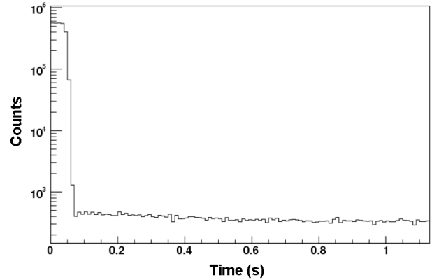
Fig. 3. Experimental DN spectrum for the 2 MeV incident neutrons on ^{232}\text{Th} .
