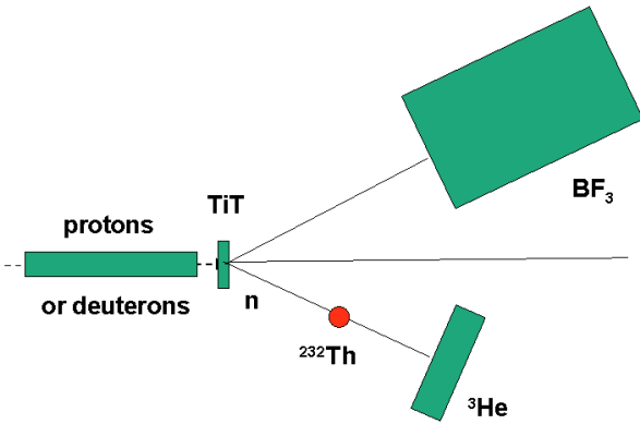
Fig. 2. Schematic view of the experiment for DN measurements from neutron induced fission.
