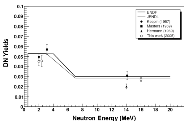
Fig. 4. Experimental data (points) and evaluations (solid lines) of DN yields as a function of neutron energy for ^{232}\text{Th} .
