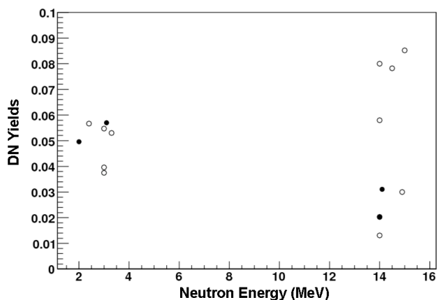
Fig. 1. Delayed neutron yield, \nu_d , data (in delayed neutrons per fission) for neutron induced fission on ^{232}\text{Th} .
